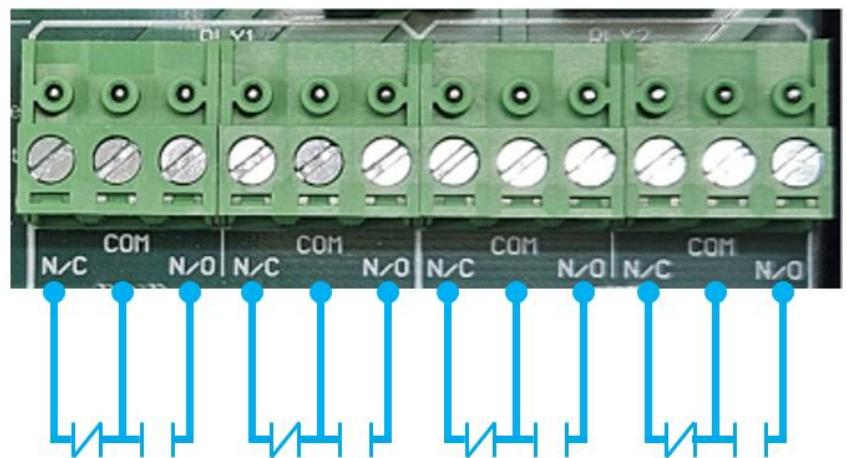
2. RLY 1 2 *NO/NC contacts 8A @ 230V 3. RLY 2 2* NO/NC contacts 8A @ 230V
