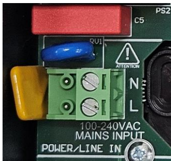
1. Power Input 100~240VAC 50-60Hz
