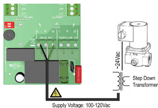
Gas Supply Controlled by 24VAC Solenoid Valve
