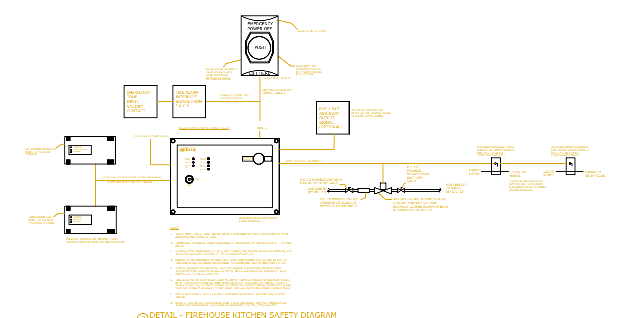
KITCHEN RANGE GAS AND ELECTRIC AND ELECTRICAL RECEPTACLES
