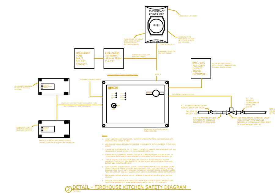
KITCHEN RANGE GAS ONLY
