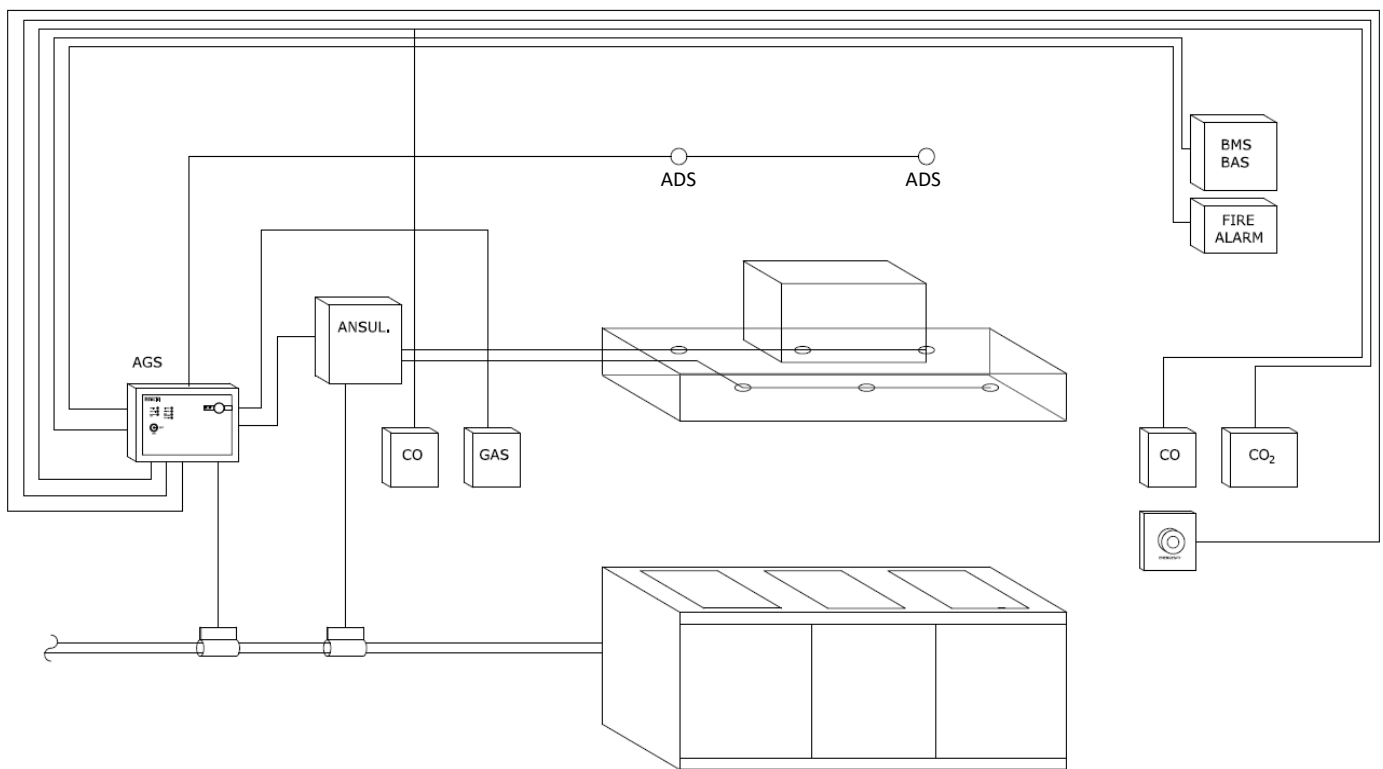
VENTILATION INTERLOCK WITH CO PROTECTION, GAS SHUT OFF & GAS PRESSURE PROVING
