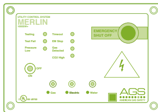
Merlin 1000SW+ Utility controller close to teachers station
