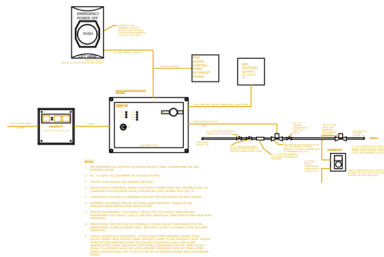
DETAIL - GAS SAFETY CONTROL FOR OUTDOOR GRILL AREA
