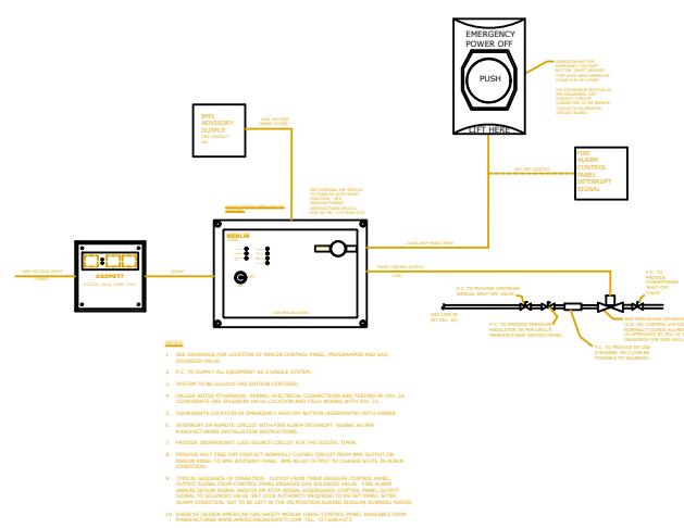
DETAIL - TIMED GAS SAFETY CONTROL FOR OUTDOOR GRILL AREA
