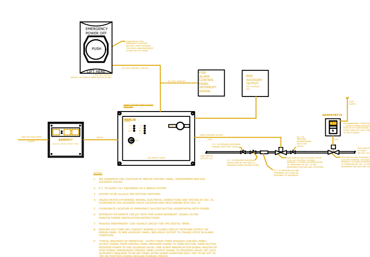
DETAIL - GAS SAFETY CONTROL FOR OUTDOOR GRILL AREA
