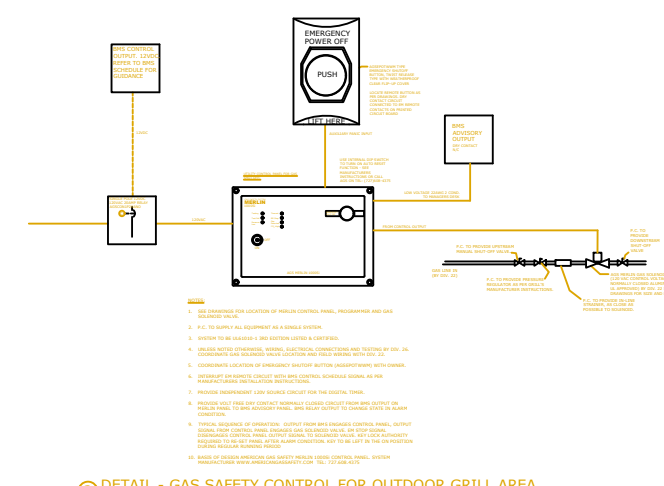
DETAIL - GAS SAFETY CONTROL FOR OUTDOOR GRILL AREA
